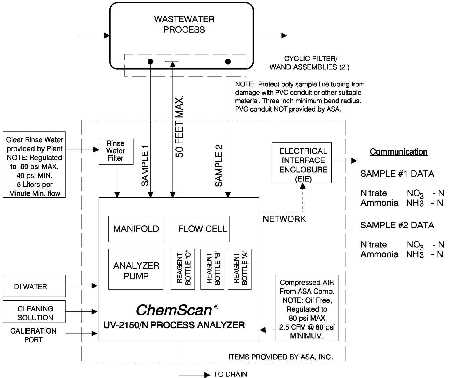
ChemScan ® Functional Block Diagram of Multiple Sample Line, Multiple Parameter, Wastewater Monitoring System
