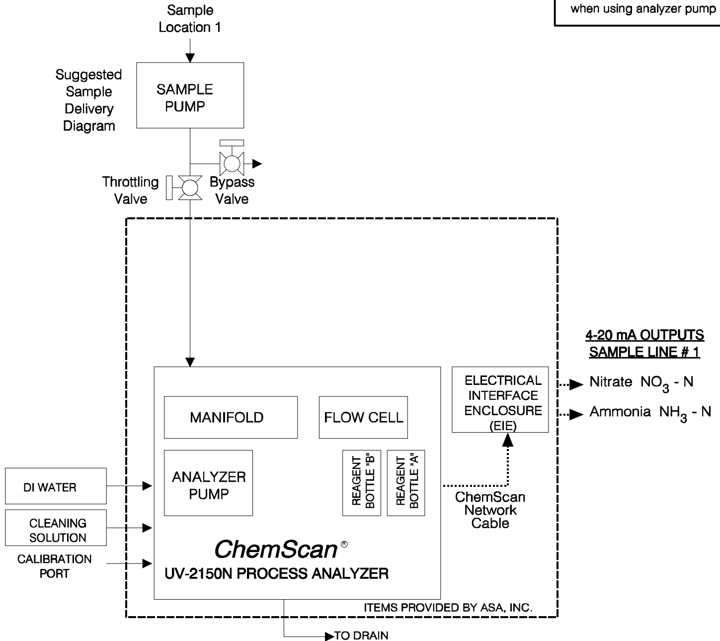
ChemScan ® Functional Block Diagram of Monitoring System
