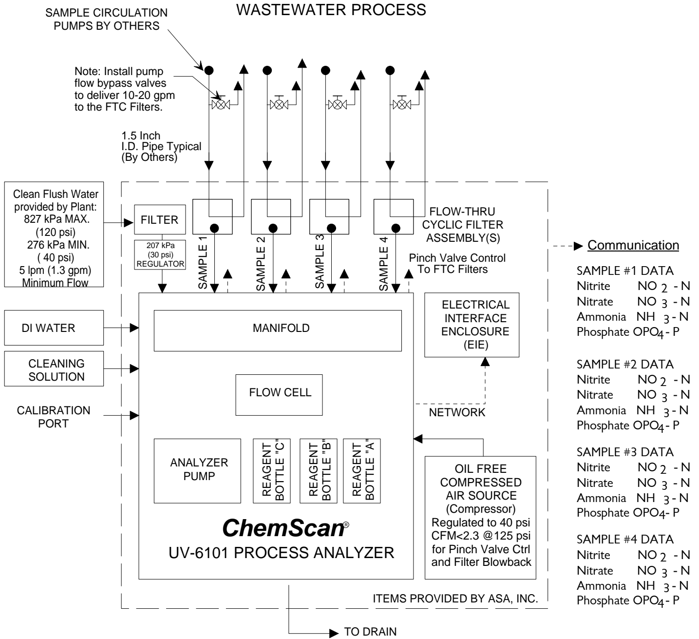
ChemScan® Functional Block Diagram of Multiple Sample Line, Multiple Parameter, Wastewater Monitoring System
