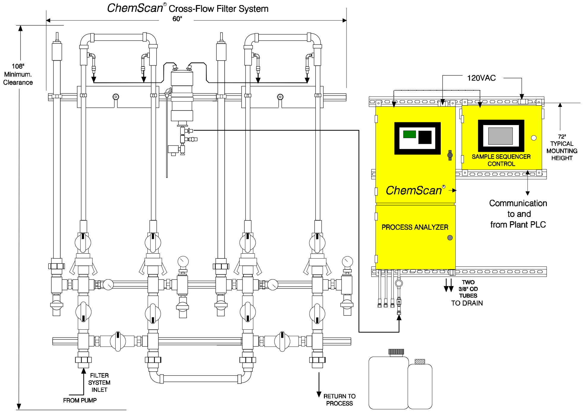
ChemScan ® System Installation Diagram - Mechanical, Plumbing, Electrical -Typical Mounting Configuration -
