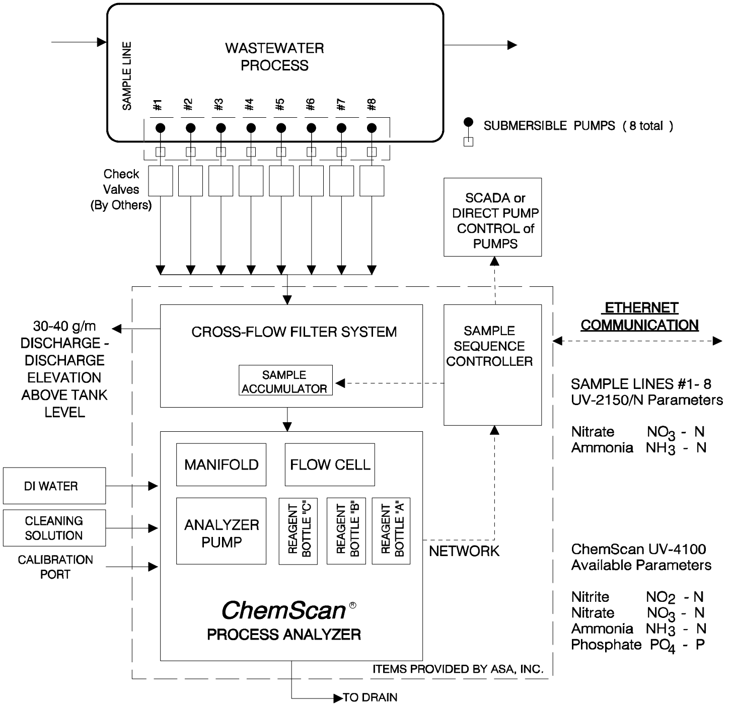
ChemScan ® Functional Block Diagram of Multi-Point, Multi-Parameter, Nutrient Analyzer System
