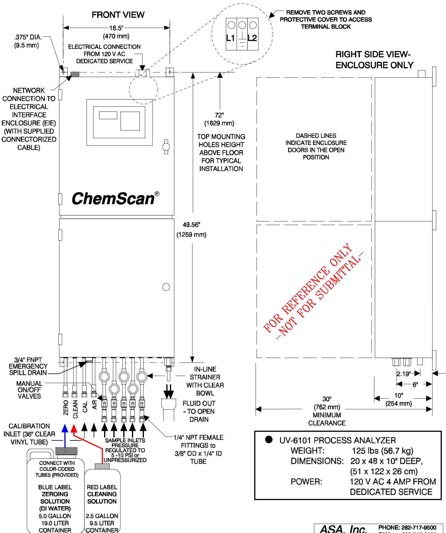
ChemScan® UV-6101 Analyzer Installation Diagram/ System Plumbing Details with Multiple Inlets and Auto Zero and Cleaning (Five Inlets Shown - Eight Maximum)
